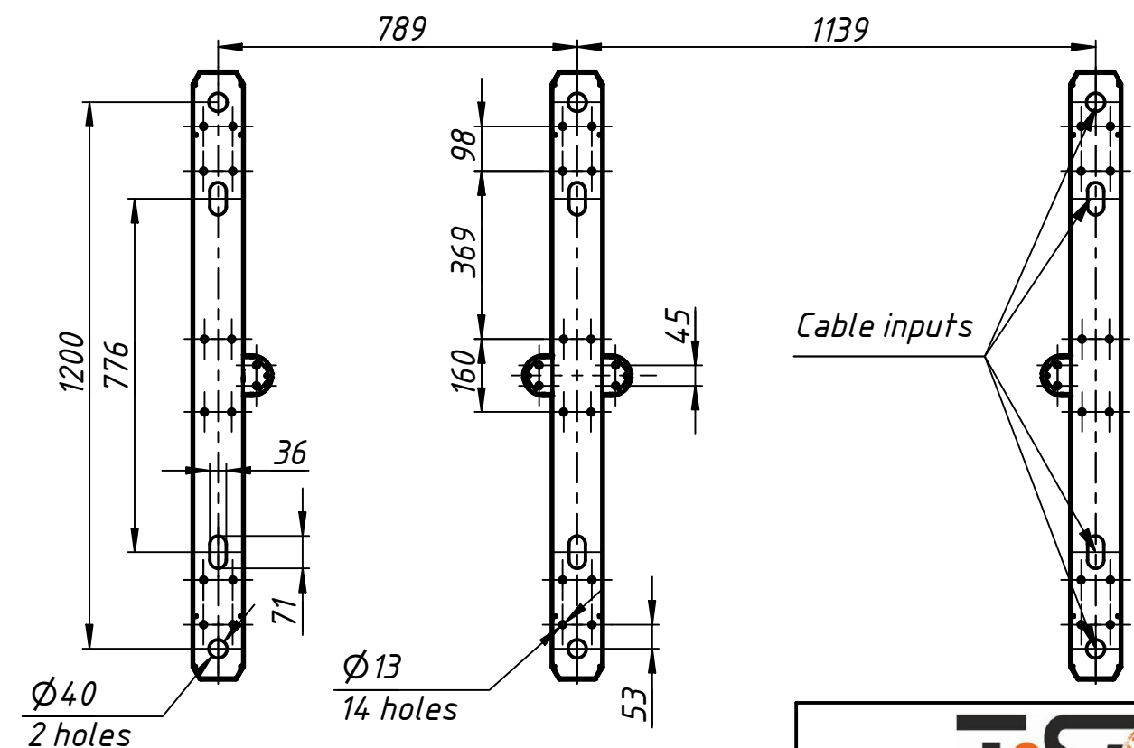
Instalation tamplate
